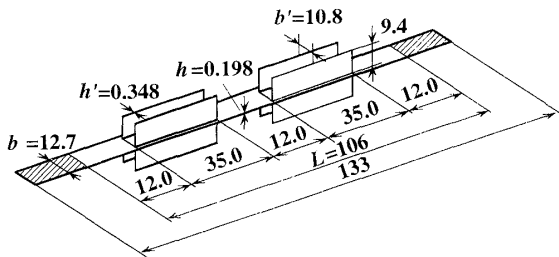
Fig. 1 Test specimen of the reinforced beam
